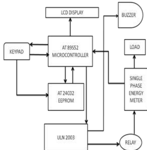
Fig.(ii) Block diagram of Prepaid energy meter
