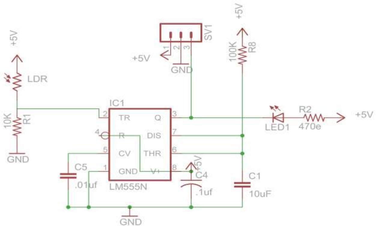
Fig.(iv) LDR Circuit
