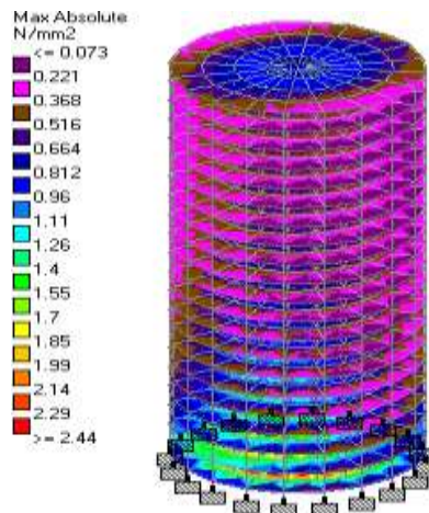
Fig 9. Maximum Absolute stress of G+20 Circular Shape Building.
