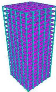
Fig 3. G+20 Square Shape Building
