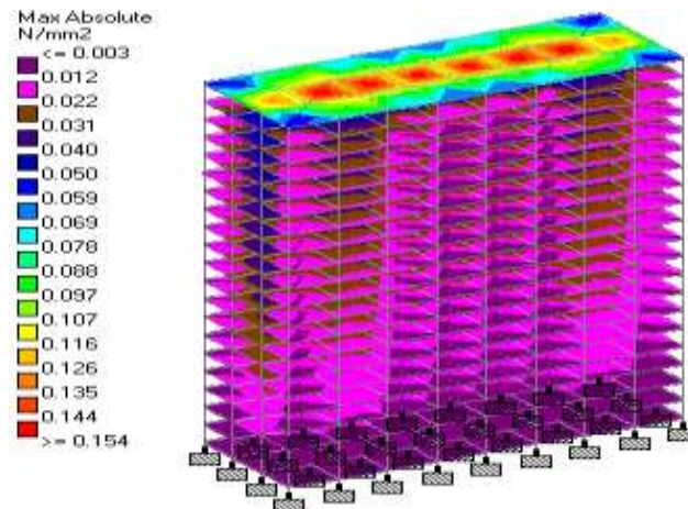
Fig 8. Maximum Absolute stress of G+20 Rectangular Shape Building.
