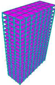
Fig 4. G+20 Rectangular Shape Building
