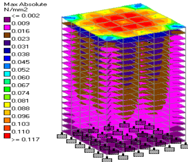
Fig 7. Maximum Absolute stress of G+20 Square Shape Building .
