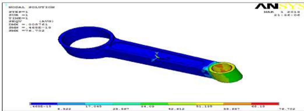
Fig 1. Structural Analysis of connecting rod I-section using Aluminium Alloy A360 ,Young's modulus - 80000MPa Poisson ratio - 0.33, Density - 0.0000026kg/mm 3
