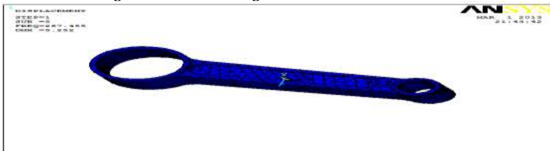
Fig 5.Modal Analysis of connecting rod I-section using Carbon Steel Young's modulus - 200000MPa,Poisson ratio - 0.295, Density - 0.000007872kg/m 3
