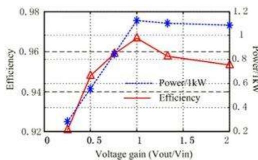
Fig.16 Efficiency versus voltage gain results corresponding to Fig. 19.
