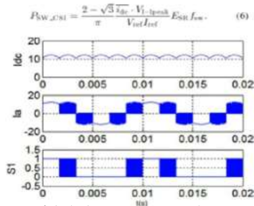
Fig. 7. Theoretic waveforms of dc-link current, output line current and switching signals.
