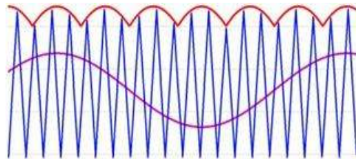
Fig.11.Variable carrier SPWM control in buck mode.
