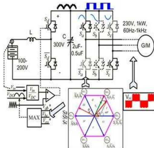
Fig. 9. SVPWAM-based boost-converter-inverter mo-tor drive system.
