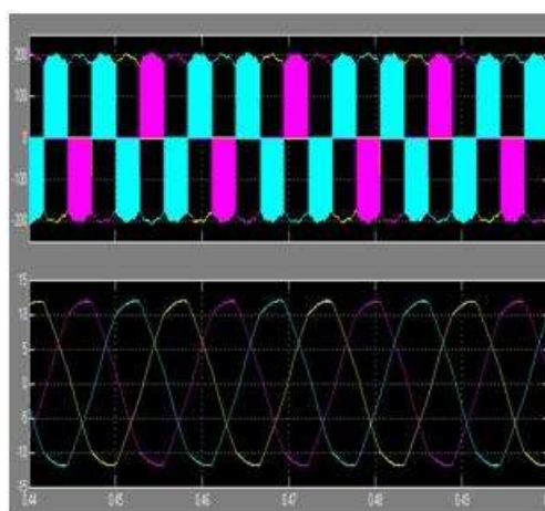
Fig.14 Inverter Output voltage and current
