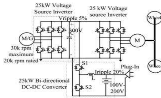
Fig 1 Typical configuration of a Fuel Cell HEV
