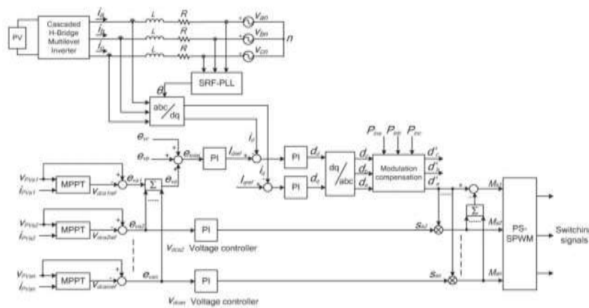
Fig.12. Control scheme for three-phase modular cascaded H-bridge multilevel PV inverter.
