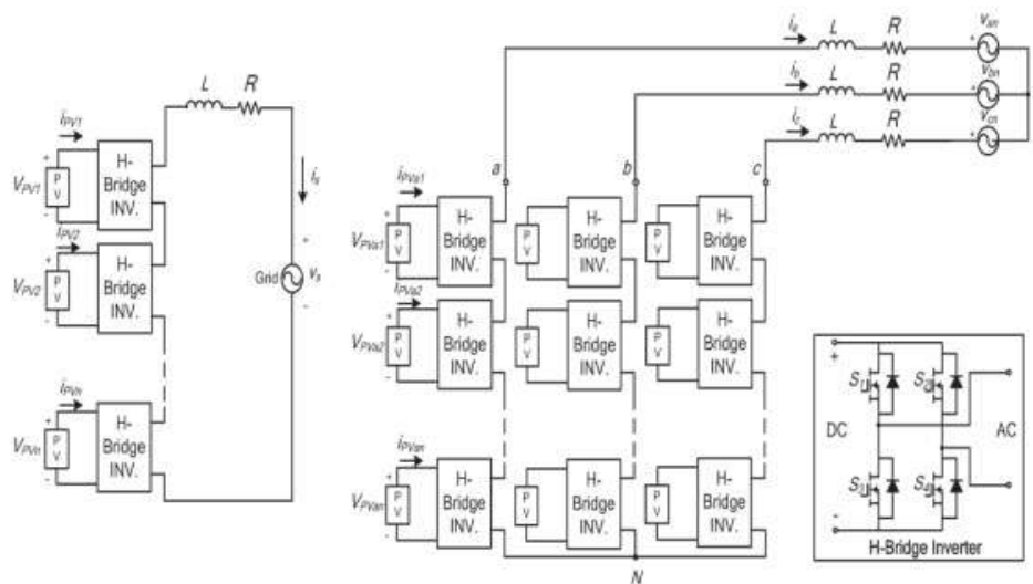
Fig.11. Topology of the modular cascaded H-bridge multilevel inverter for grid-connected PV systems.
