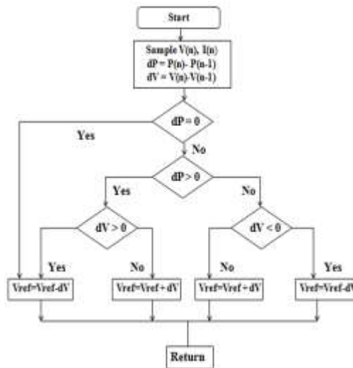
Fig.3.Flow chart of perturb and observe
