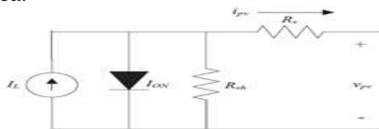
Fig.2. Equivalent circuit diagram of the PV cell
