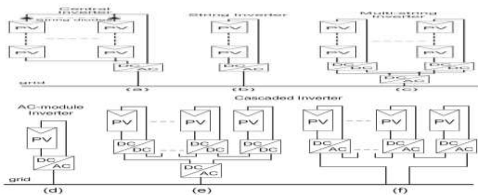
Fig. 1. Configurations of PV systems. (a) Central inverter.
